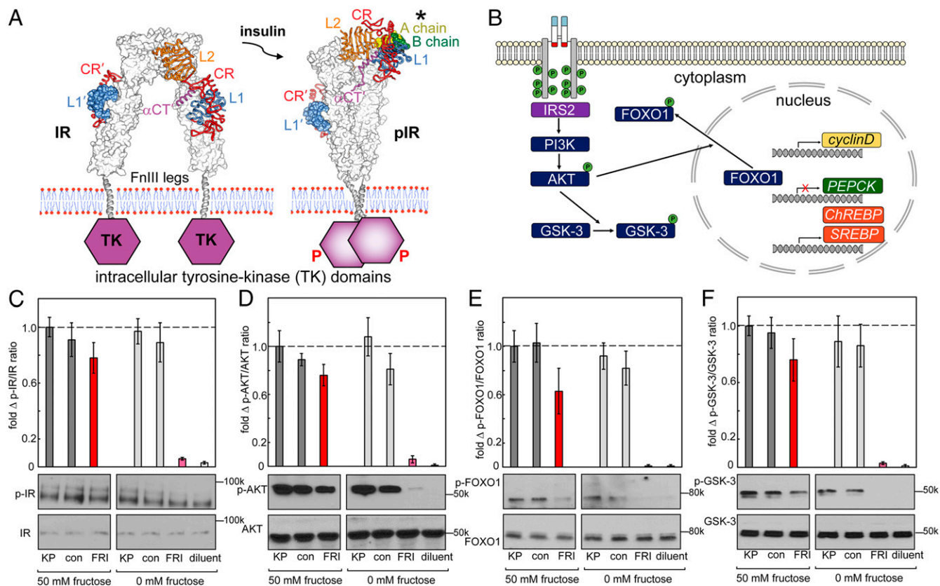
Fig. 4. Fructose-dependent IR activation and downstream pathways. (A) IR ectodomain structures either unbound ( Left ) or as activated by insulin ( Right ), asterisk highlights the A chain (light green) and B chain (green) of insulin. On insulin binding, the ectodomain legs come together to enable TK transphosphorylation (red P's). (B) Selected downstream IR signaling pathways as probed by WB. IR L1 and \alpha CT domains are highlighted in blue and red; JM- and TK-domain phosphorylation sites are shown in schematic form by green circles. IR activation leads to AKT phosphorylation, which in turn phosphorylates and inhibits GSK-3; pAKT also phosphorylates FOXO in cytoplasm to enable transcriptional regulation of cell proliferation ( cyclin D ), gluconeogenesis ( PEPCK ), and fatty-acid synthesis ( ChREBP and SREBP ) in the nucleus. (C-F) WB assays probing the p-IR/IR (C), p-AKT/AKT (D), p-FOXO/FOXO (E), and p-GSK-3/GSK-3 (F) in the presence or absence of fructose (50 mM) in medium. Studies of FRI were conducted relative to lispro insulin ("KP"), a diol-free control analog (DFC; "con") or buffer only (diluent; "dil"). The error bars in histograms indicate SEM. Representative gel images are displayed underneath corresponding columns in histograms; assays were performed in triplicate.
